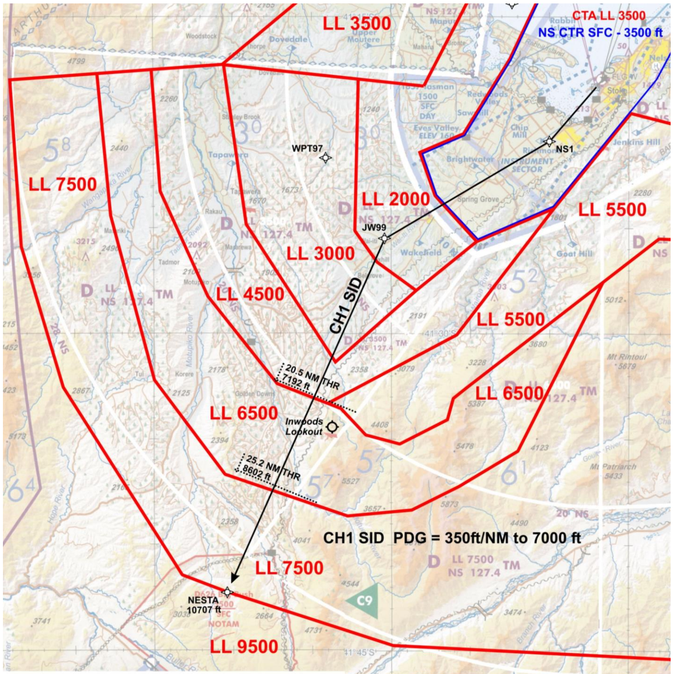
Diagram 12 Draft CTA to the south with the RWY 20 departure to NZCH.
