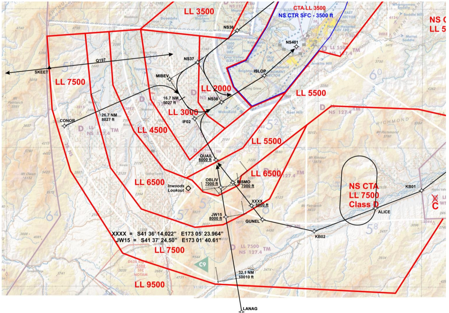
Diagram 11 Draft CTA to the south with arrivals from NZCH, NZWN and the West Coast along with the RNAV approach to RWY 02. The planned new 'ALICE' holding pattern on the RWY 02 arrival from the east is also depicted. The CTA LL 7500 ft is expanded south to correctly contain this new holding pattern.
