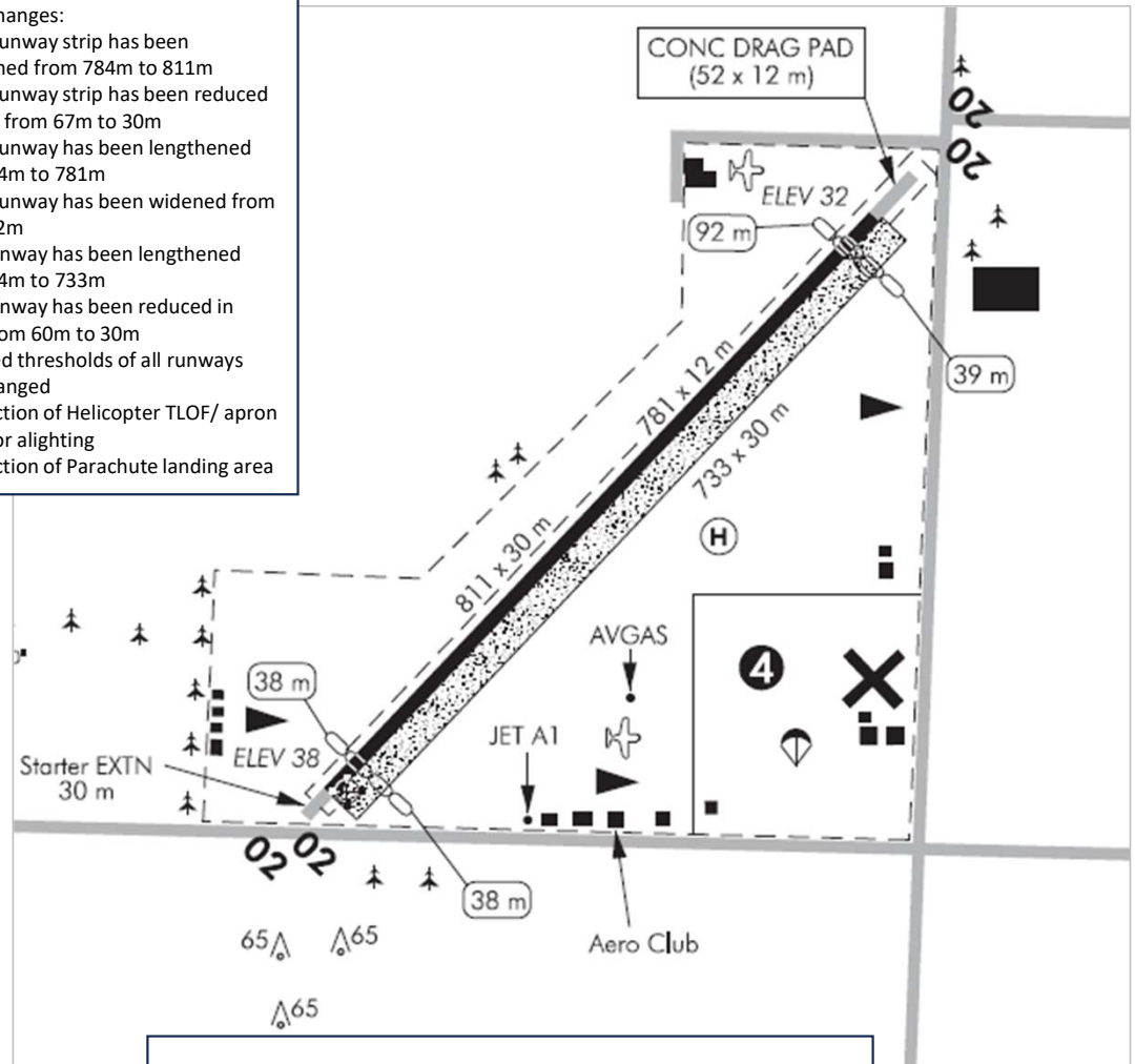
Aerodrome layout – Eff 1 Dec 22
